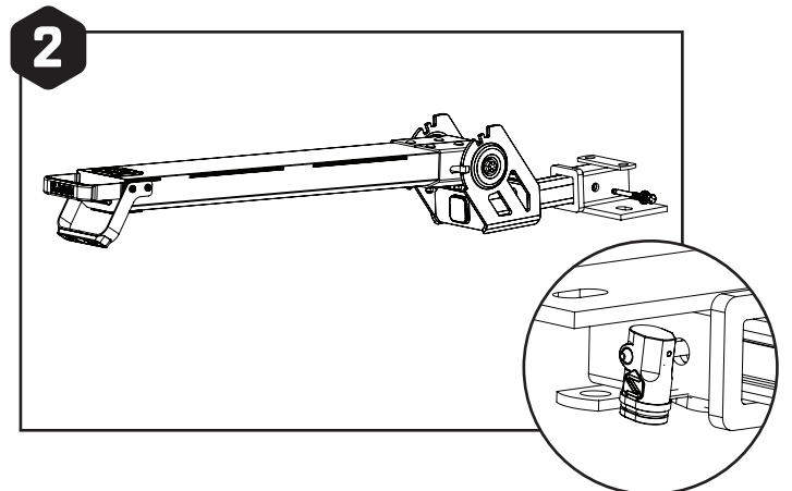
Insert MHS base into receiver. Line up hitch pin holes. Apply grease to hitch pin threads before installing rack to vehicle. Reapply as needed to prevent corrosion. Insert hitch pin through the passenger side. Tighten with 5/8" wrench. Lift up on base while tightening for a secure install. Rack may settle after initial use. Check and re-tighten as needed. A properly tightened rack will have no movement inside the vehicle receiver. Insert grey lock head on to hitch pin. Lock will work in either direction.
